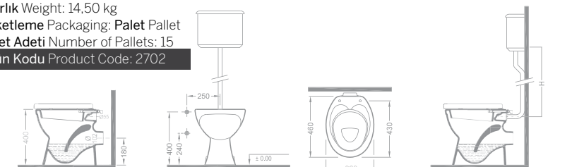
Klozet Arkadan | Single WC Pan - P trap
